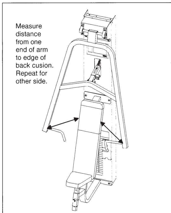
Figure 1 - Verifying Alignment
